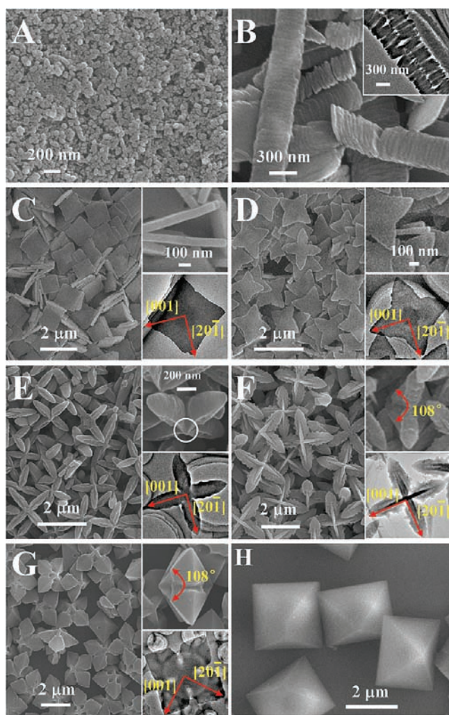
Figure 5. SEM images of ZnTPP·H 2 O ONCs prepared at C_{\text{ZnTPP}} = (A) 0.143 (particles), (B) 0.167 (square flakes), (C) 0.200 (square flakes), (D) 0.222 (planar tetrapods), (E) 0.250 (crosses), (F) 0.333 (hexapods), (G) 0.500 (growing octahedrons), and (H) 0.667 mM (octahedrons), respectively, in the presence of PVP (fixed at 0.1 M in repeating units in all the reaction mixtures) as the capping ligand. The inset in (B) is the TEM image of 1D self-assembly of square nanoflakes. The right top and bottom insets in (C)–(G) are the corresponding high-magnification SEM and TEM images, respectively.
