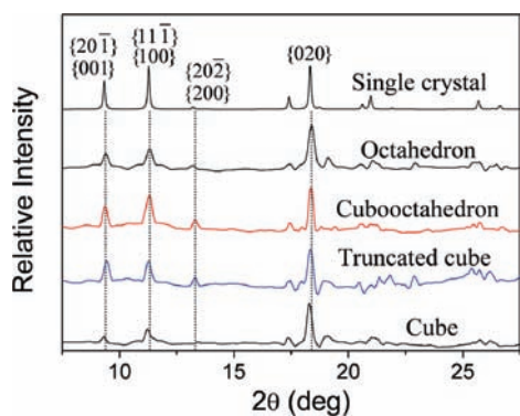
Figure 2. XRD patterns of cubes, truncated cubes, cubooctahedrons, and octahedrons, prepared in the presence of CTAB surfactant. The top line shows the standard powder spectrum simulated on the basis of the single crystal data by using the DIAMOND software.
